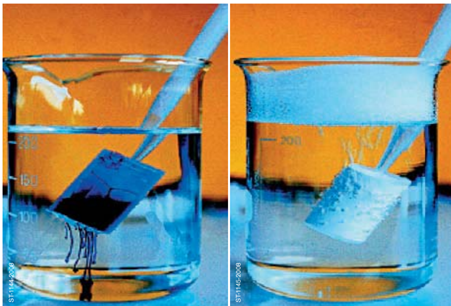
Demonstration of pressure compensation Immersion in warm water: on the left, chemicals released due to positive pressure; on the right, effective compensation of positive pressure without damage to the sensor.
